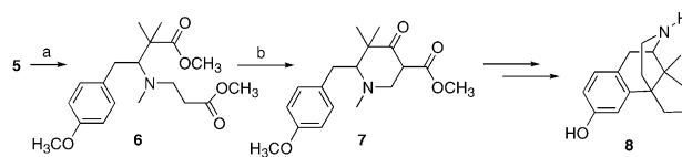
Scheme 2. Reagents: (a) methyl acrylate, cat. HOAc, HCOOH, HCHO; (b) NaH, toluene.
