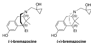
Figure 1. Absolute stereochemistry of breamazocine enantiomers.
