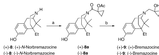
Scheme 3. Reagents: (a) 1-Acetoxycyclopropanecarboxylic acid, EDCI, CH 2 Cl 2 ; (b) LiAlH 4 , H 2 SO 4 , THF.
