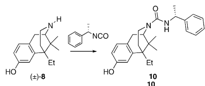
Scheme 4. Diastereomeric urea formation employing R -(+)-1-phenylethylisocyanate.
